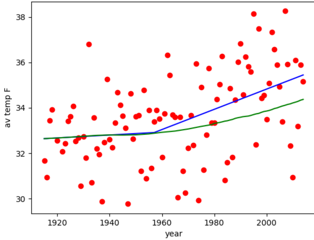
Kr Tavmean vs. CO2 1957
