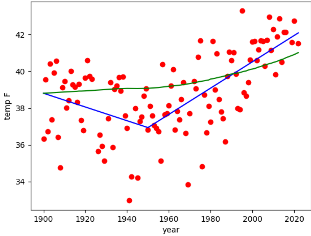
Kazan 1950 tavmean vs co2
